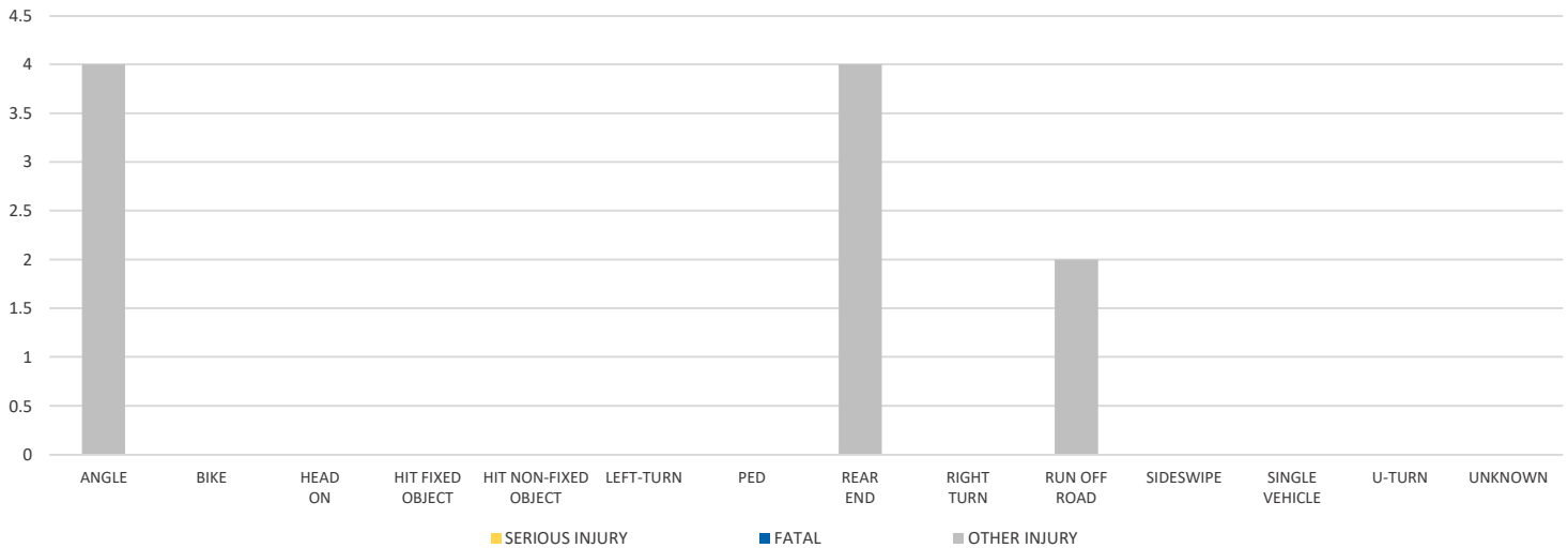
CRASH TYPE
