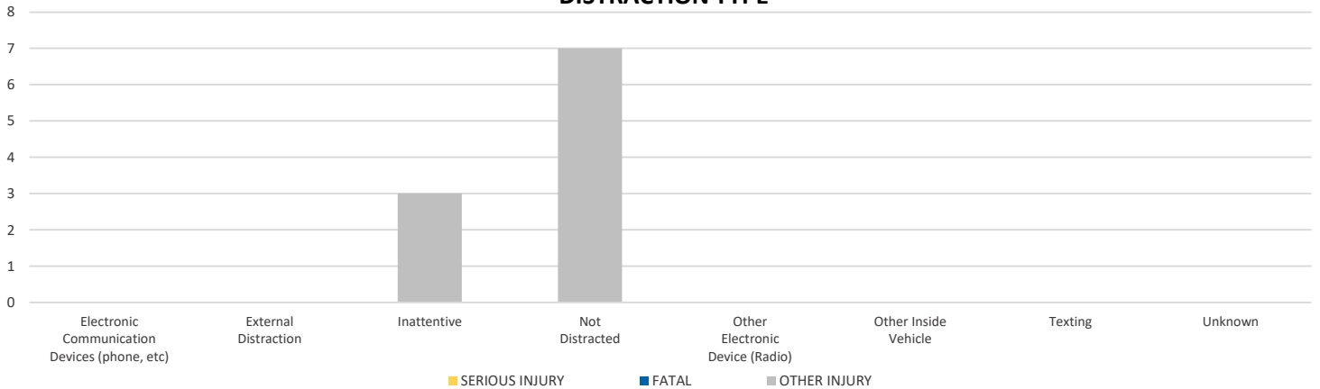
DISTRACTION TYPE
